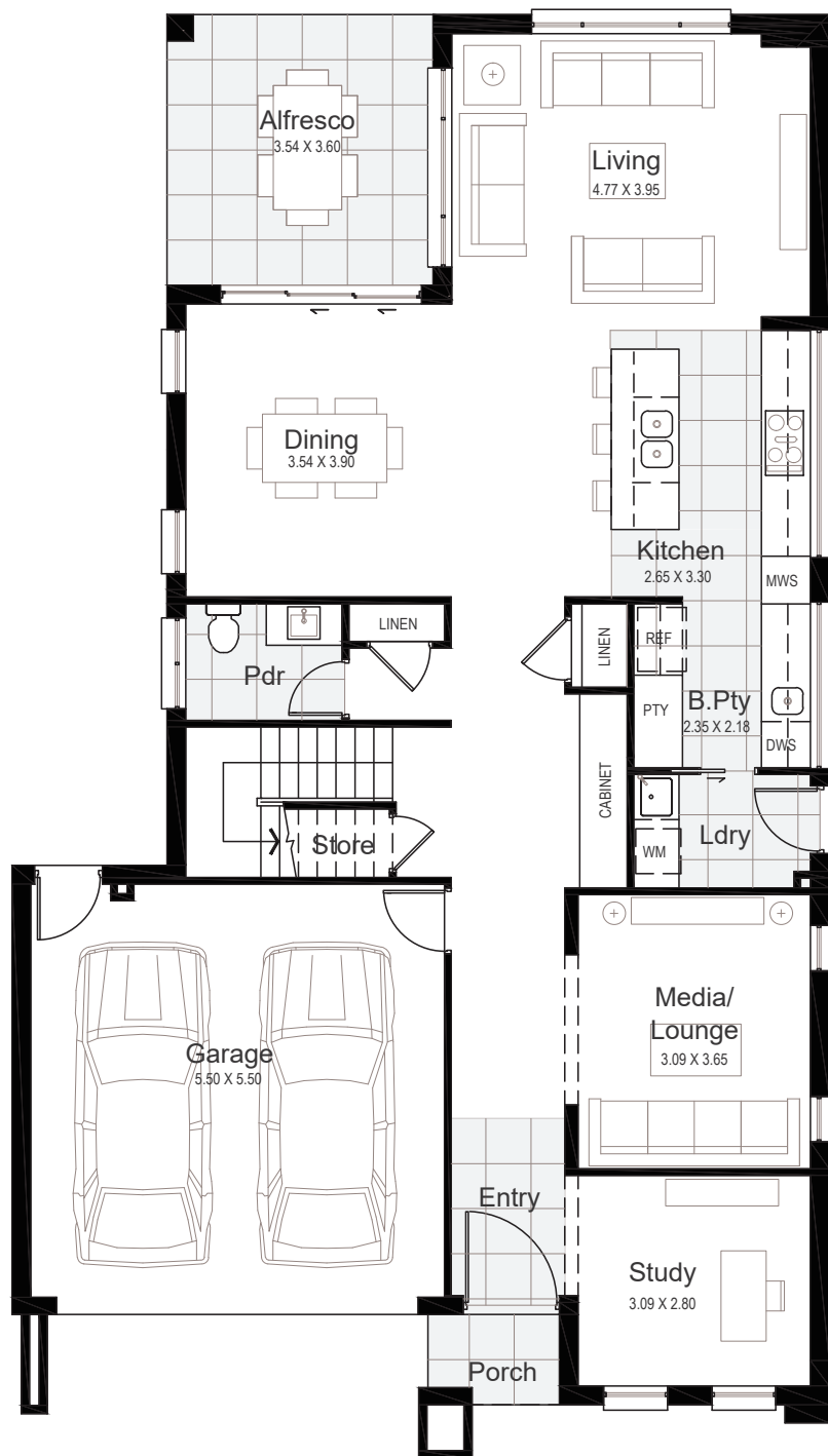
Ground Floor
